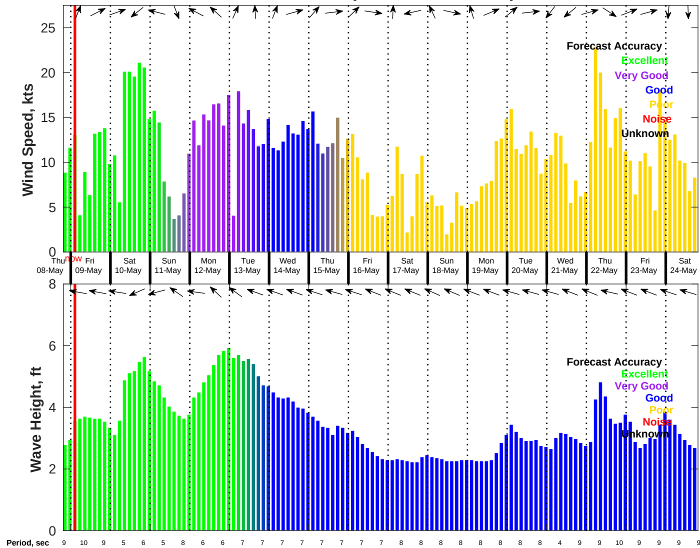
Wind & Wave Forecast for NDBC 41004 from 08-May-2025 19:00:00 to 24-May-2025 19:00:00
