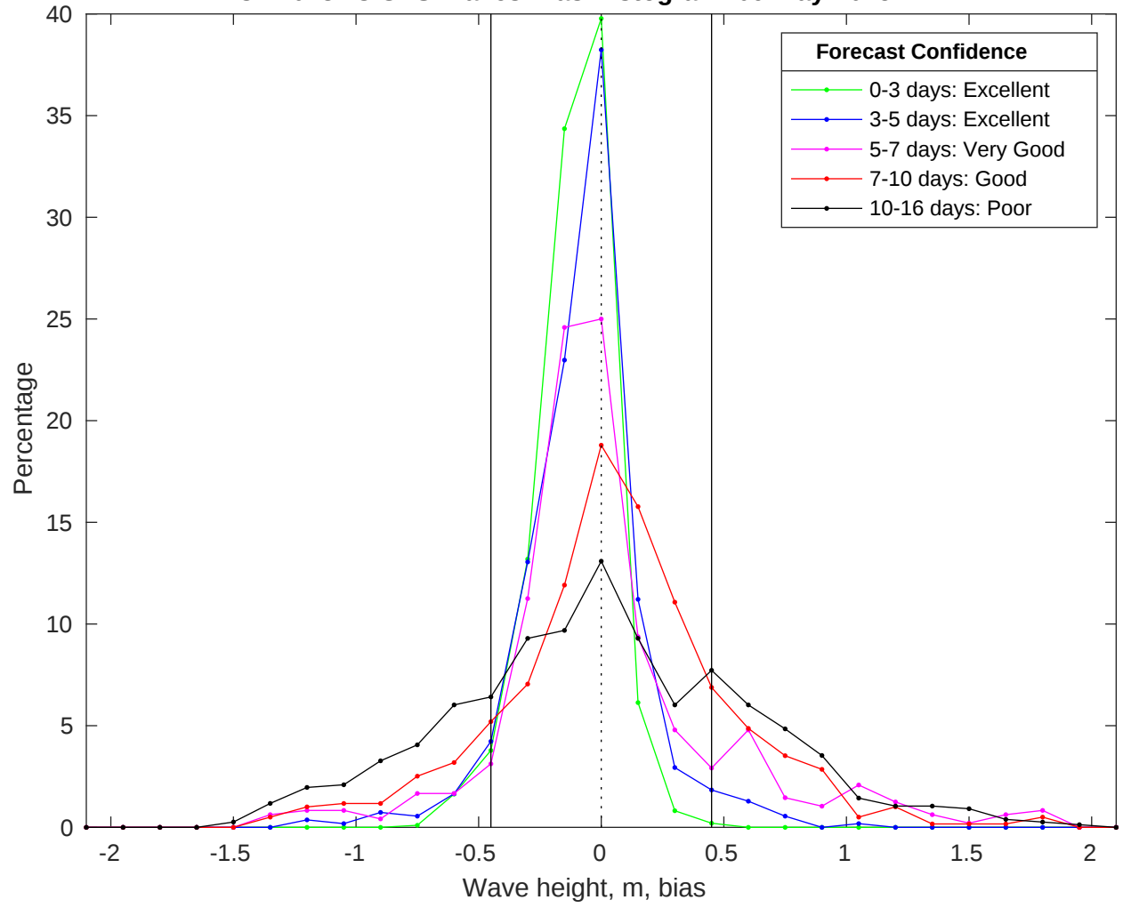
NDBC 41013 vs GFS Waves Bias Histogram: 09-May-2025
