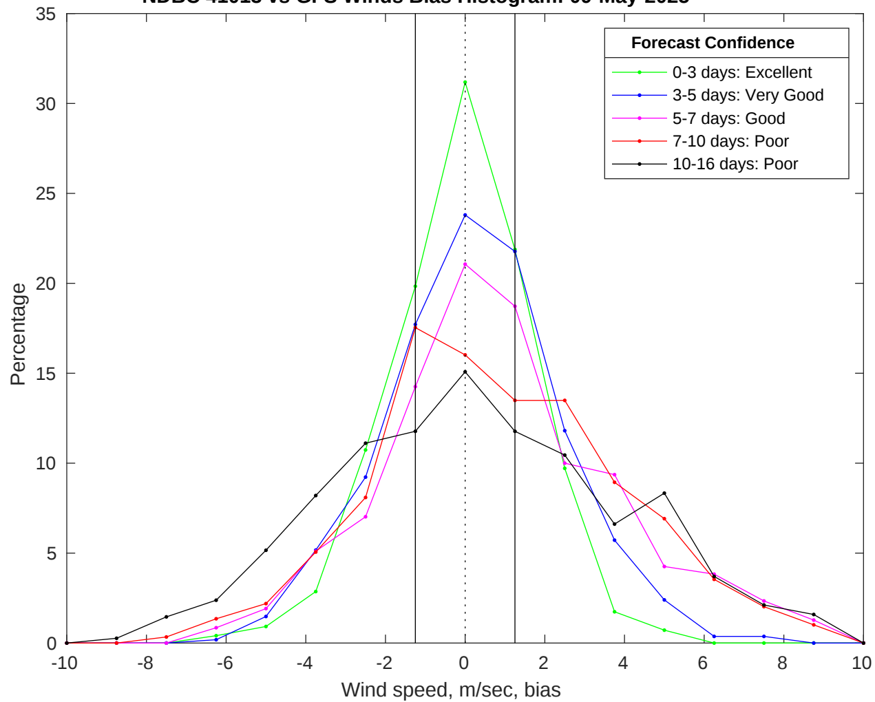
NDBC 41013 vs GFS Winds Bias Histogram: 09-May-2025
