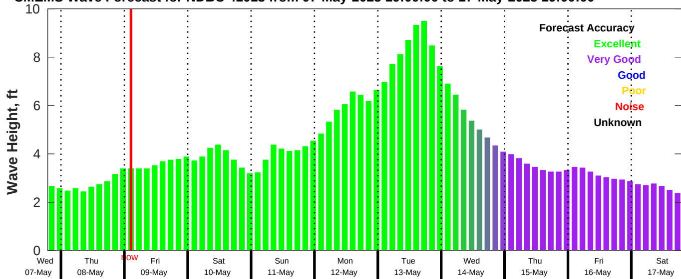
CMEMS Wave Forecast for NDBC 41013 from 07-May-2025 19:00:00 to 17-May-2025 19:00:00
