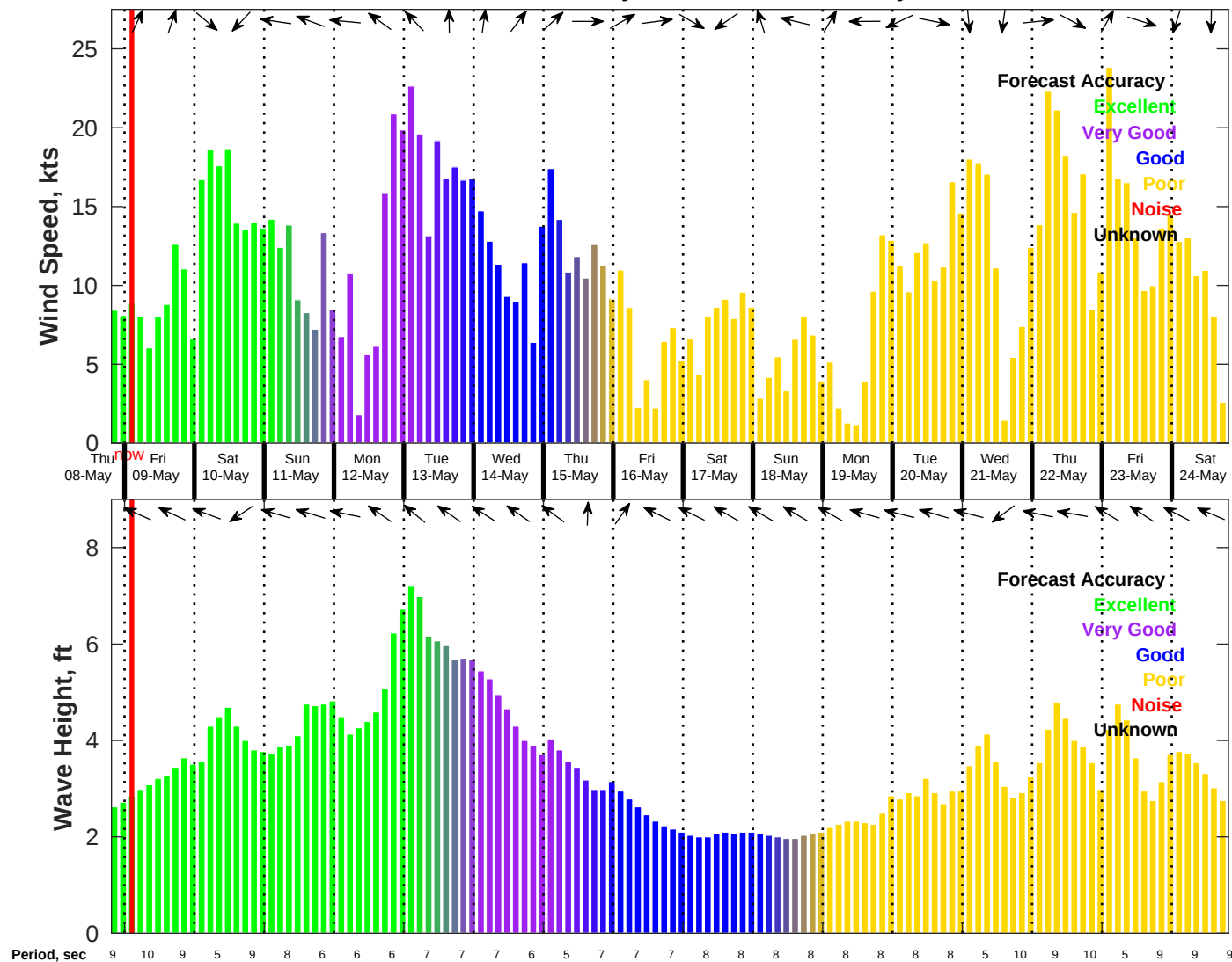
Wind & Wave Forecast for NDBC 41013 from 08-May-2025 19:00:00 to 24-May-2025 19:00:00
