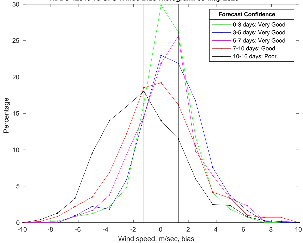
NDBC 42019 vs GFS Winds Bias Histogram: 09-May-2025
