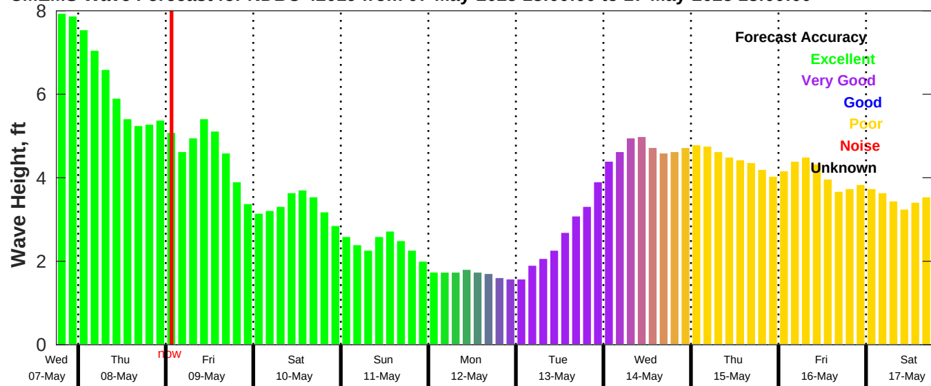
CMEMS Wave Forecast for NDBC 42019 from 07-May-2025 18:00:00 to 17-May-2025 18:00:00
