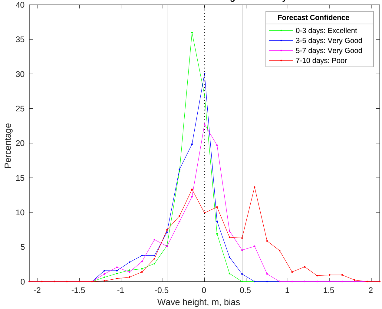
NDBC 42020 vs CMEMS Waves Bias Histogram: 09-May-2025
