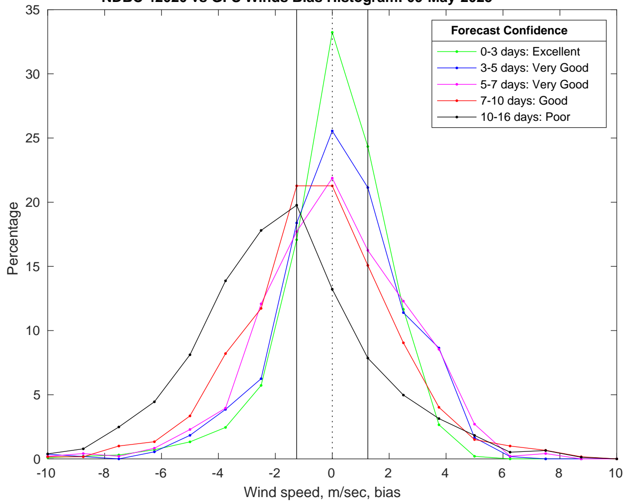
NDBC 42020 vs GFS Winds Bias Histogram: 09-May-2025
