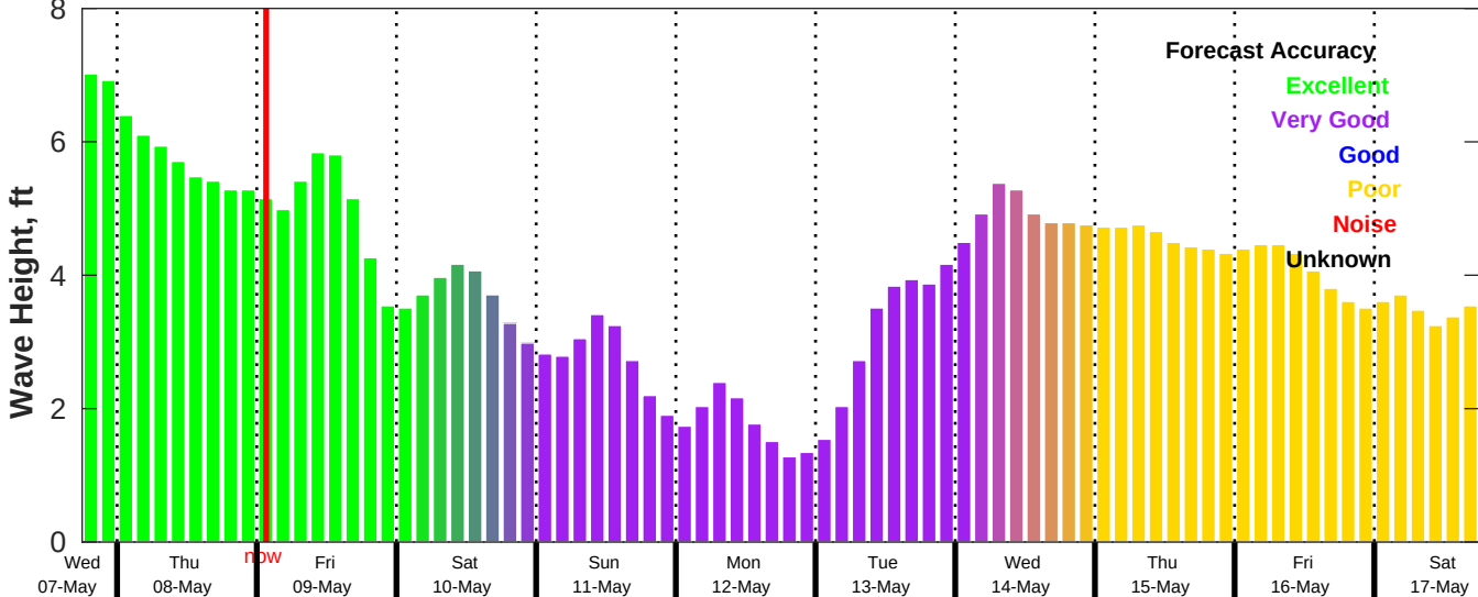
CMEMS Wave Forecast for NDBC 42020 from 07-May-2025 18:00:00 to 17-May-2025 18:00:00
