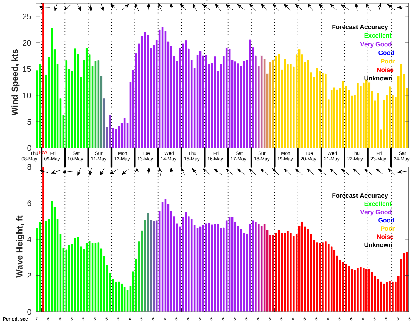
Wind & Wave Forecast for NDBC 42020 from 08-May-2025 18:00:00 to 24-May-2025 18:00:00
