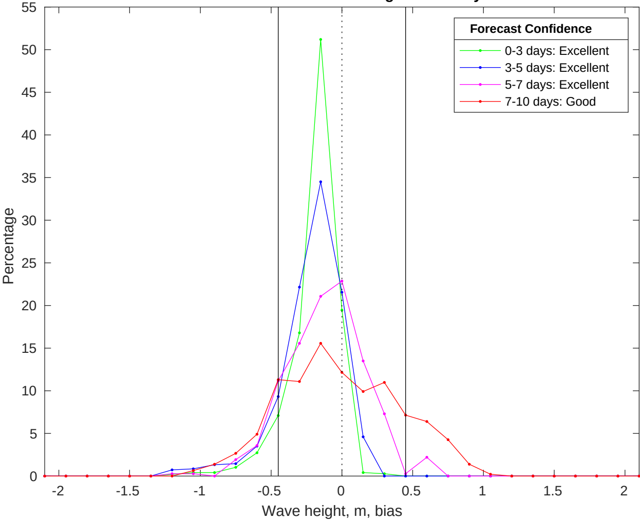
NDBC 42035 vs CMEMS Waves Bias Histogram: 09-May-2025
