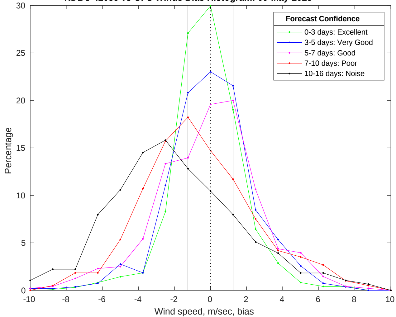
NDBC 42035 vs GFS Winds Bias Histogram: 09-May-2025
