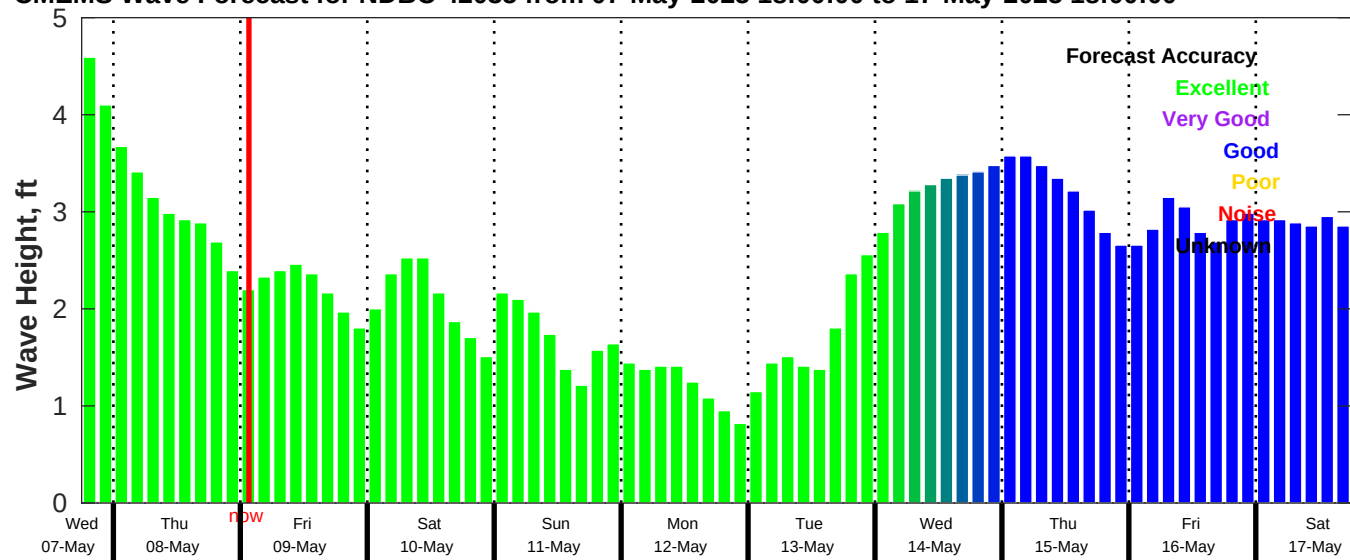
CMEMS Wave Forecast for NDBC 42035 from 07-May-2025 18:00:00 to 17-May-2025 18:00:00
