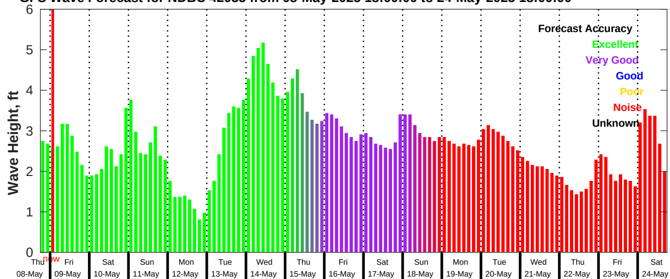
GFS Wave Forecast for NDBC 42035 from 08-May-2025 18:00:00 to 24-May-2025 18:00:00
