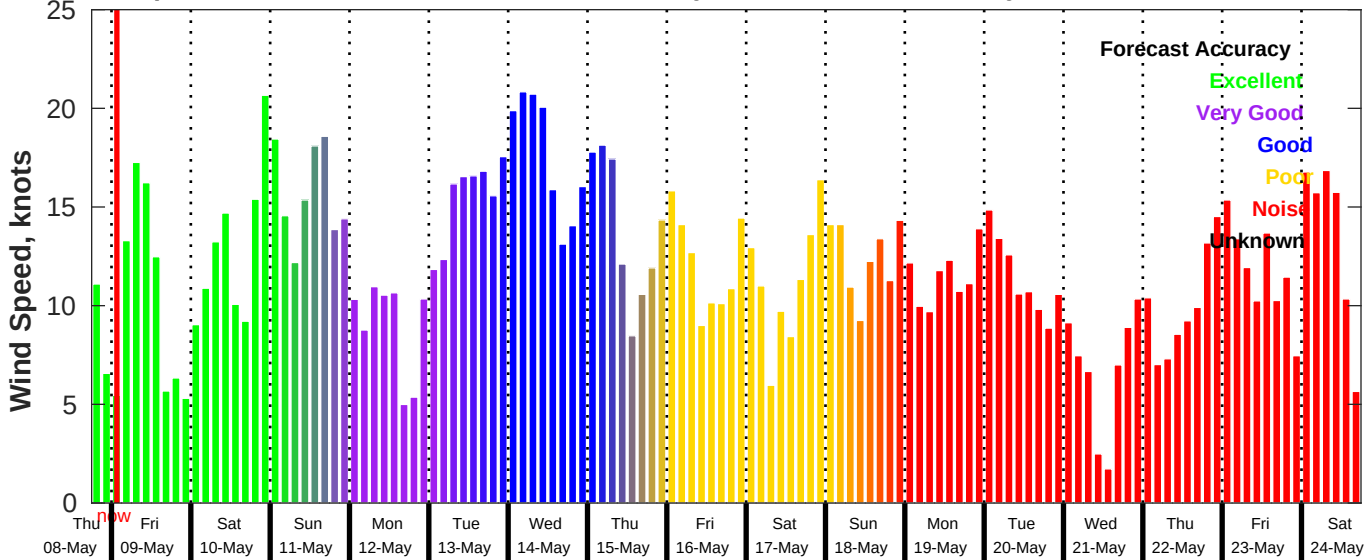
GFS Wind Speed Forecast for NDBC 42035 from 08-May-2025 18:00:00 to 24-May-2025 18:00:00
