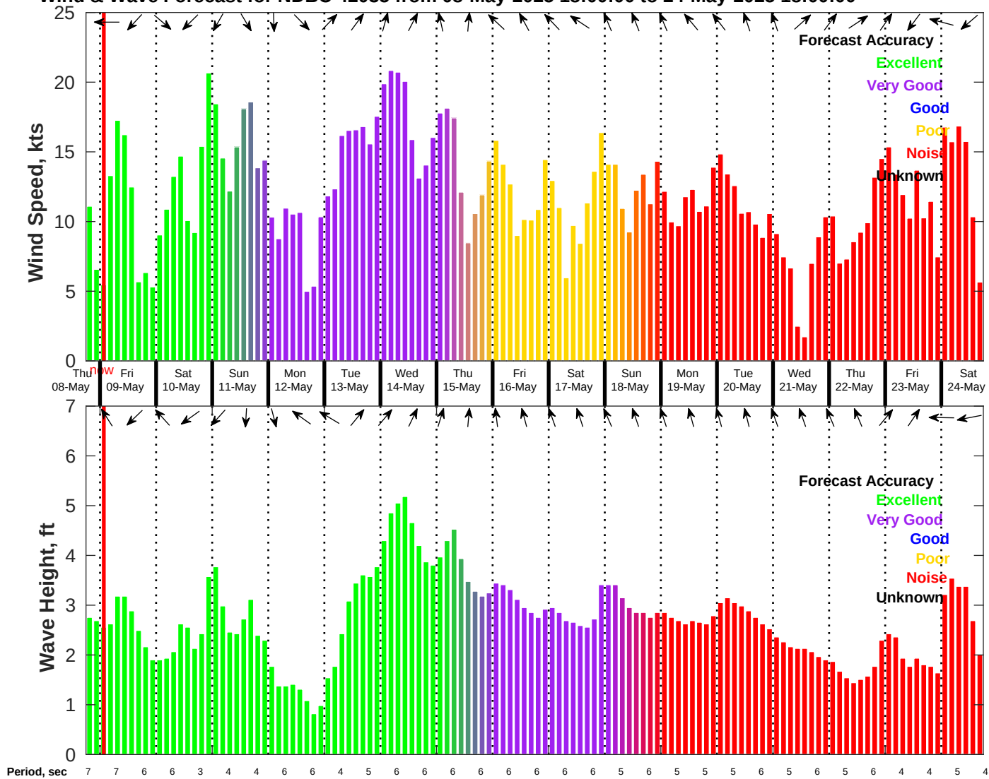
Wind & Wave Forecast for NDBC 42035 from 08-May-2025 18:00:00 to 24-May-2025 18:00:00
