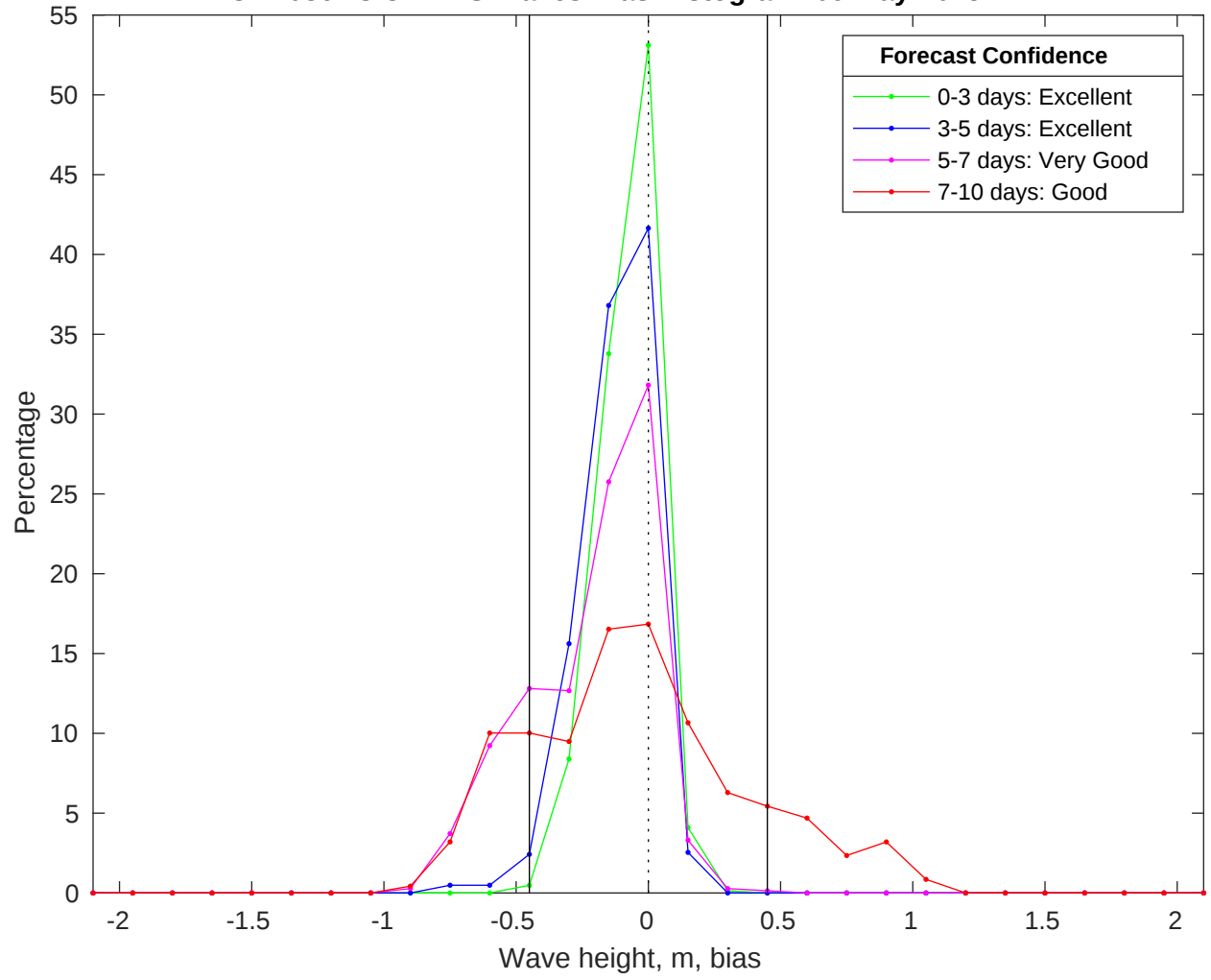
NDBC 42036 vs CMEMS Waves Bias Histogram: 09-May-2025
