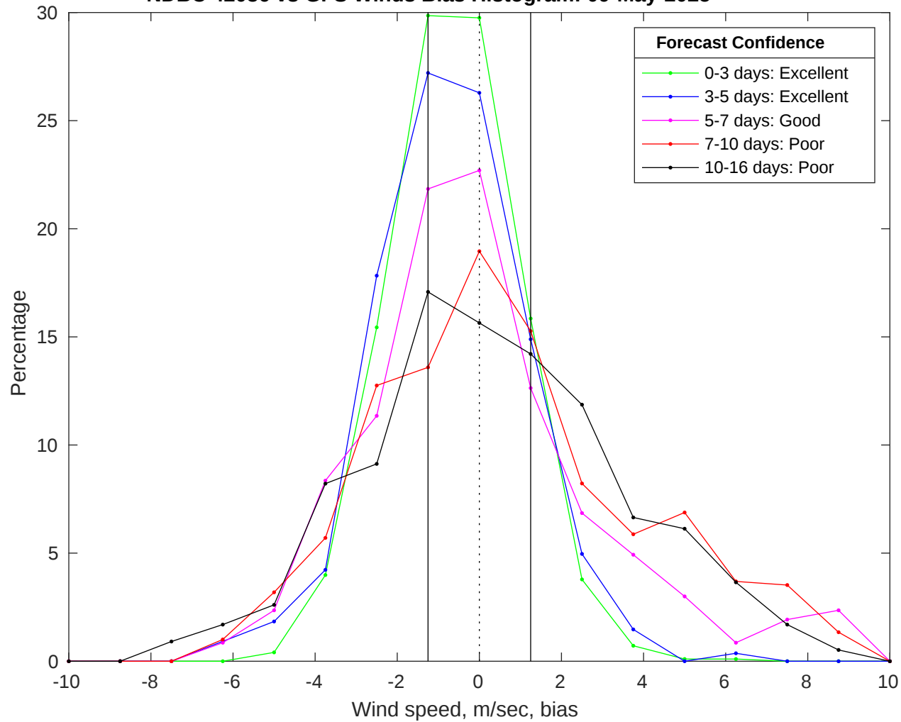
NDBC 42036 vs GFS Winds Bias Histogram: 09-May-2025
