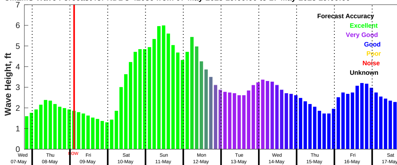
CMEMS Wave Forecast for NDBC 42036 from 07-May-2025 19:00:00 to 17-May-2025 19:00:00
