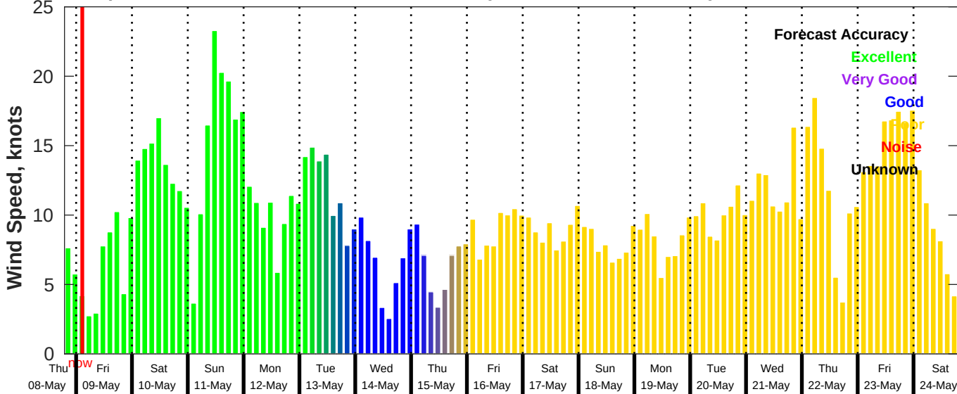
GFS Wind Speed Forecast for NDBC 42036 from 08-May-2025 19:00:00 to 24-May-2025 19:00:00
