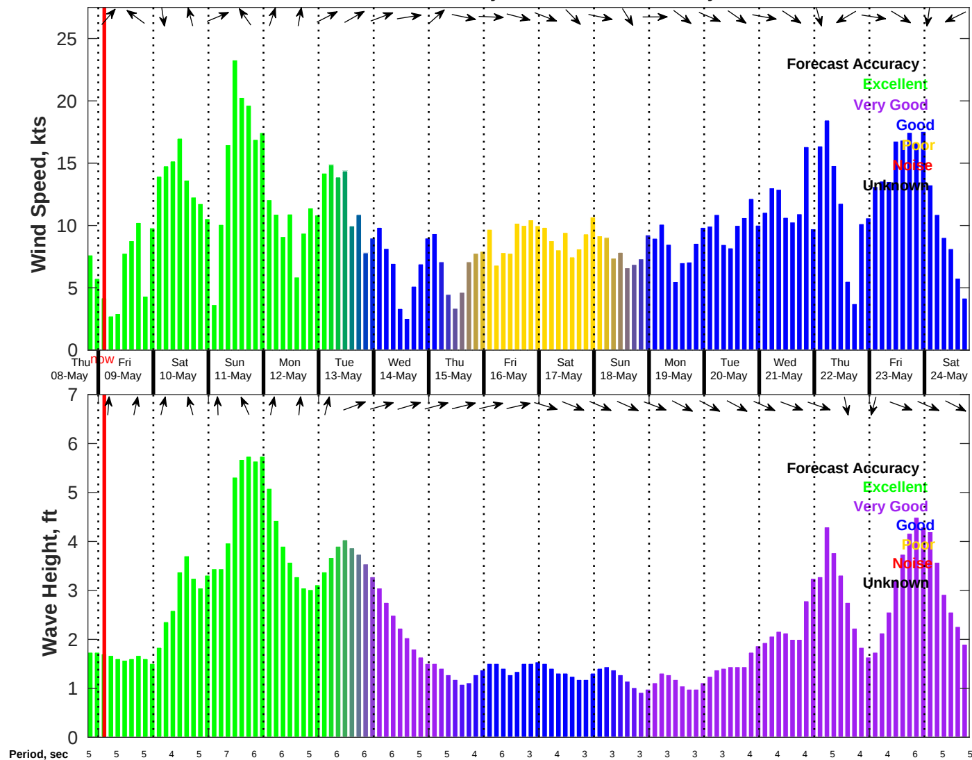
Wind & Wave Forecast for NDBC 42036 from 08-May-2025 19:00:00 to 24-May-2025 19:00:00
