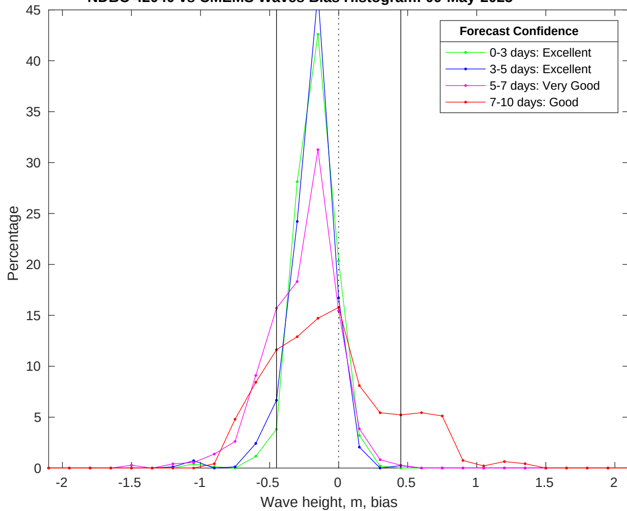
NDBC 42040 vs CMEMS Waves Bias Histogram: 09-May-2025
