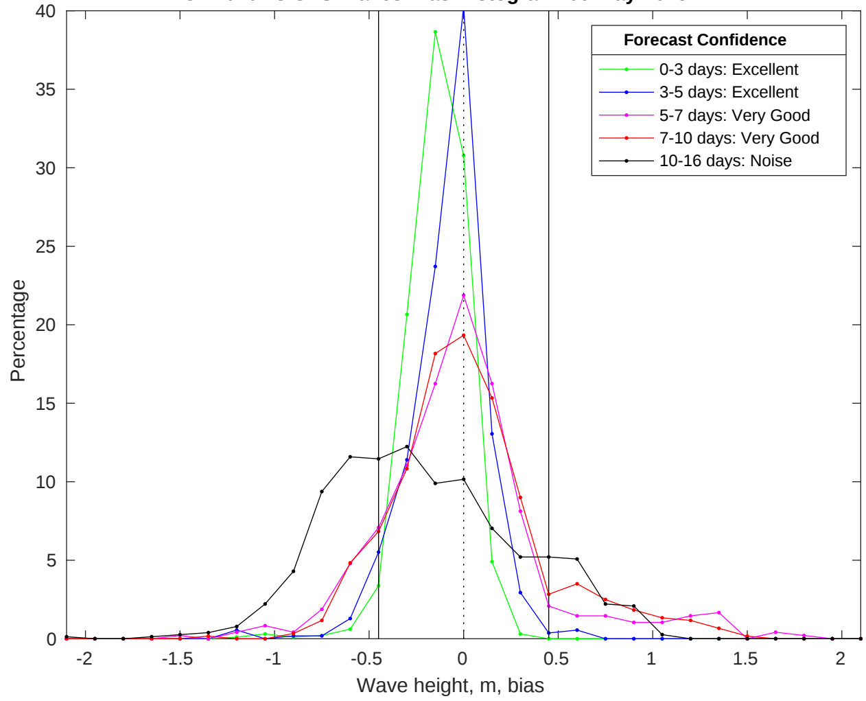
NDBC 42040 vs GFS Waves Bias Histogram: 09-May-2025
