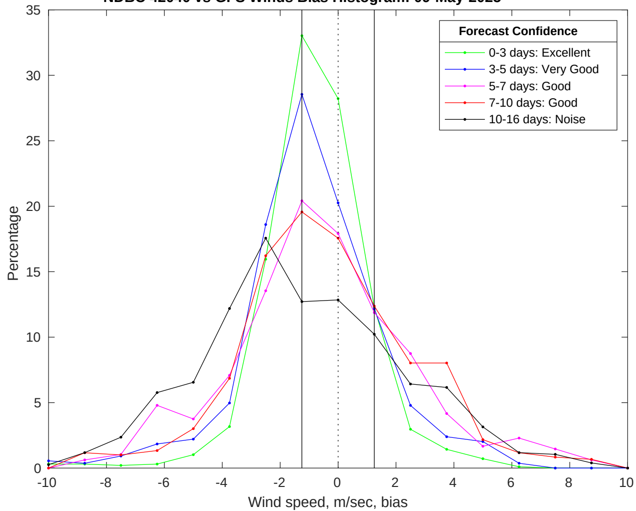
NDBC 42040 vs GFS Winds Bias Histogram: 09-May-2025
