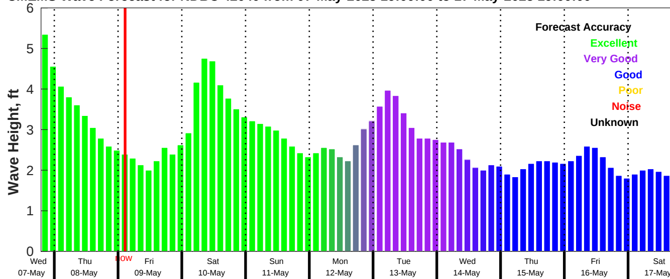
CMEMS Wave Forecast for NDBC 42040 from 07-May-2025 19:00:00 to 17-May-2025 19:00:00
