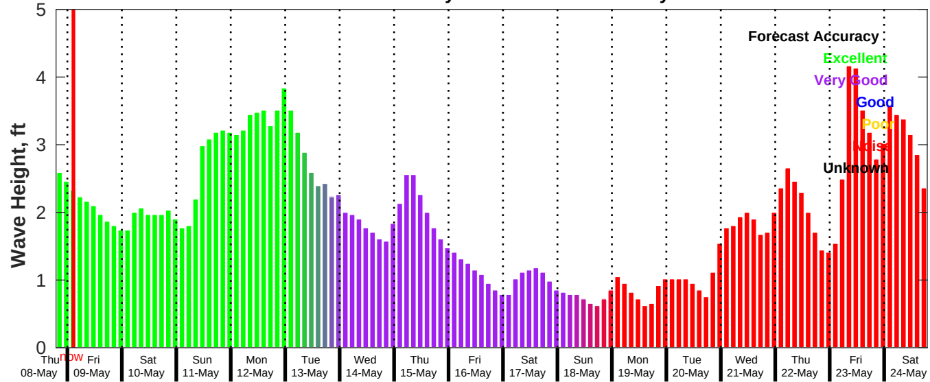
GFS Wave Forecast for NDBC 42040 from 08-May-2025 19:00:00 to 24-May-2025 19:00:00
