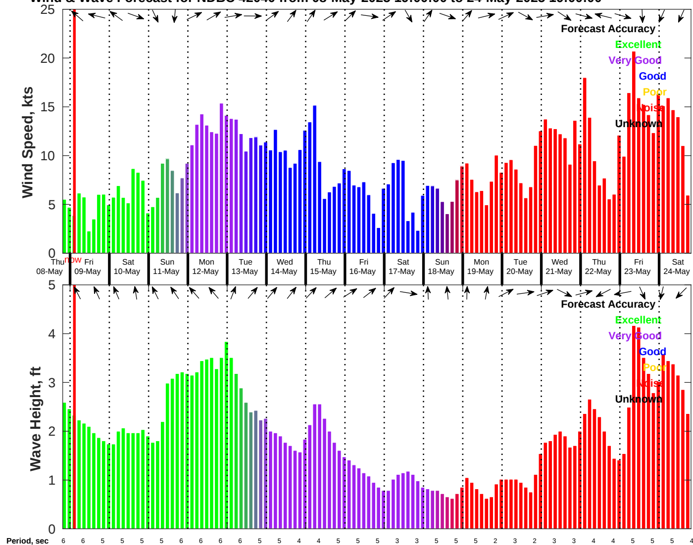
Wind & Wave Forecast for NDBC 42040 from 08-May-2025 19:00:00 to 24-May-2025 19:00:00
