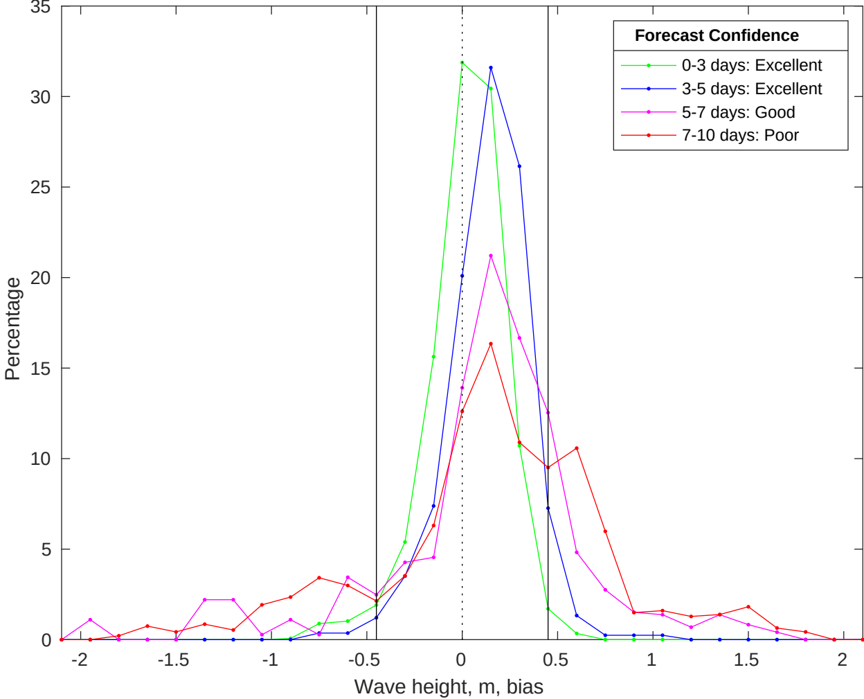
NDBC 46011 vs CMEMS Waves Bias Histogram: 09-May-2025
