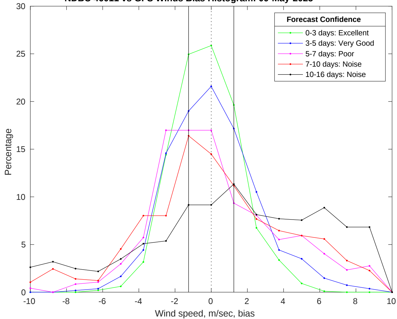
NDBC 46011 vs GFS Winds Bias Histogram: 09-May-2025
