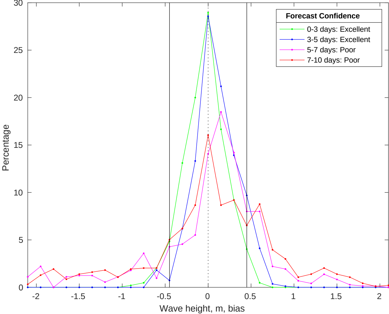
NDBC 46028 vs CMEMS Waves Bias Histogram: 09-May-2025
