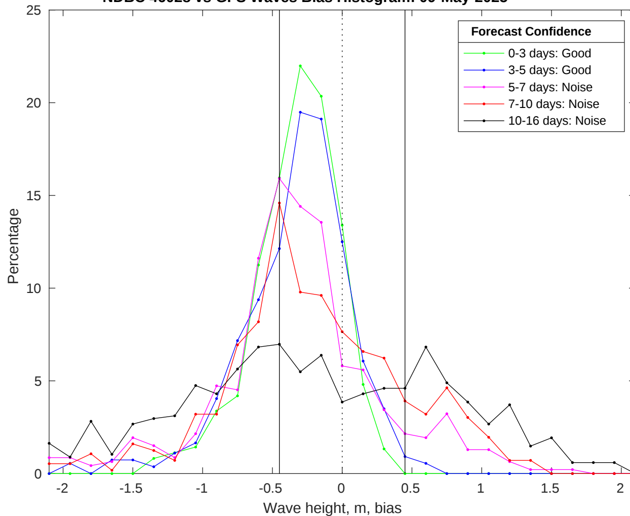
NDBC 46028 vs GFS Waves Bias Histogram: 09-May-2025
