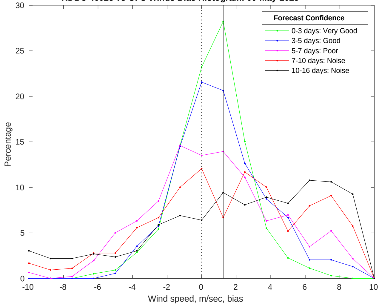
NDBC 46028 vs GFS Winds Bias Histogram: 09-May-2025
