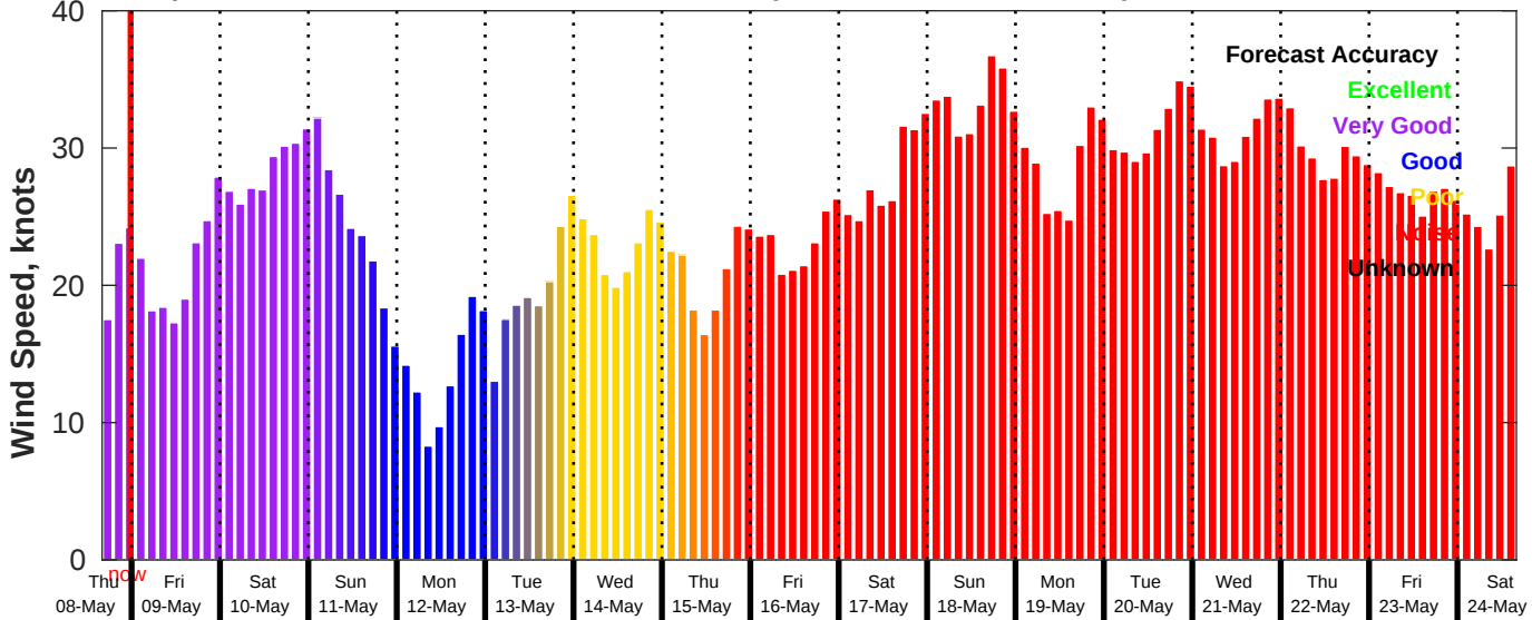
GFS Wind Speed Forecast for NDBC 46028 from 08-May-2025 16:00:00 to 24-May-2025 16:00:00
