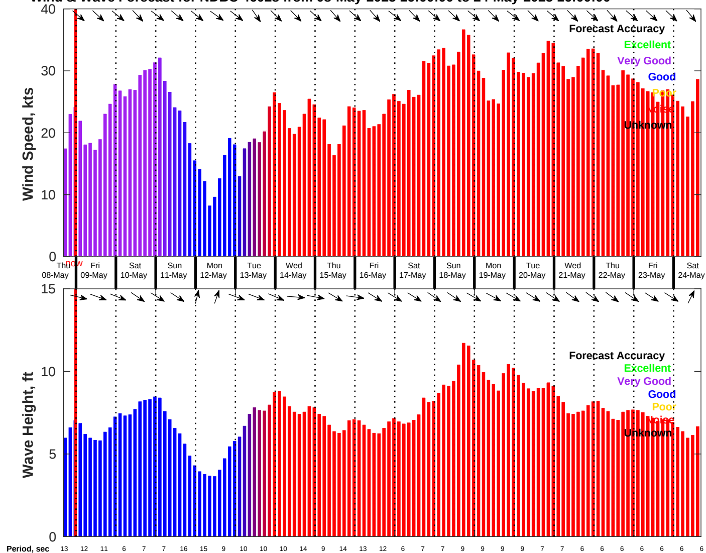
Wind & Wave Forecast for NDBC 46028 from 08-May-2025 16:00:00 to 24-May-2025 16:00:00
