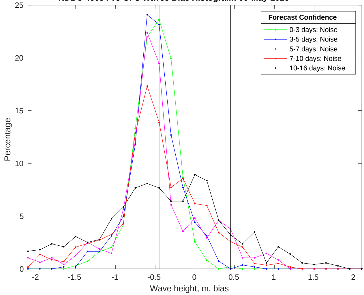
NDBC 46054 vs GFS Waves Bias Histogram: 09-May-2025
