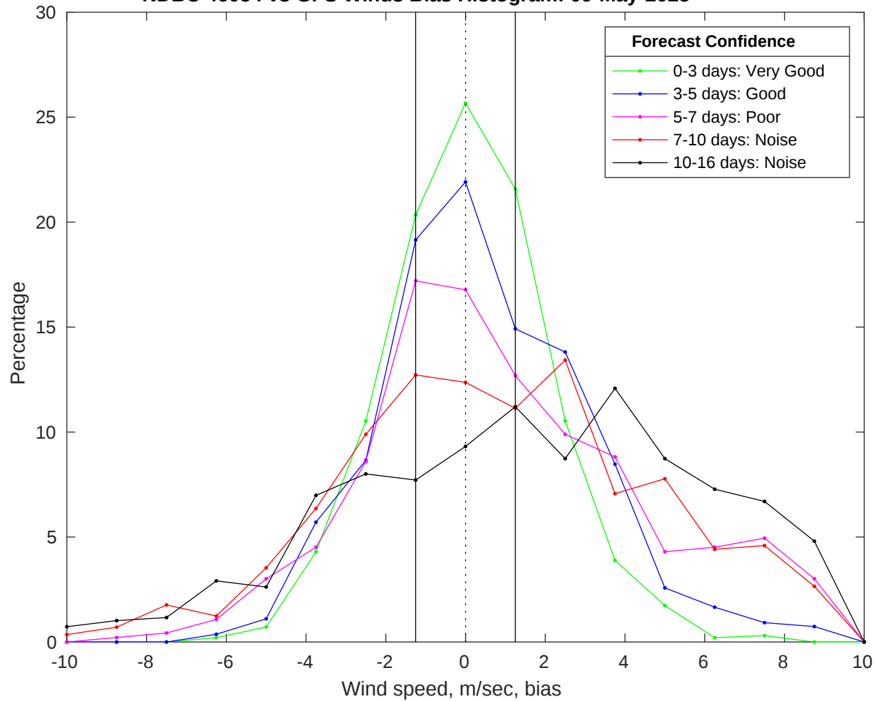
NDBC 46054 vs GFS Winds Bias Histogram: 09-May-2025
