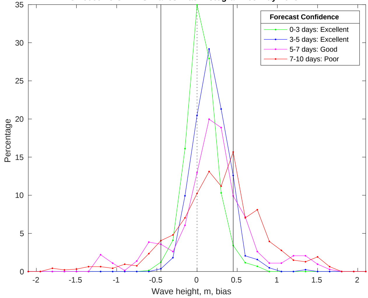
NDBC 46069 vs CMEMS Waves Bias Histogram: 09-May-2025
