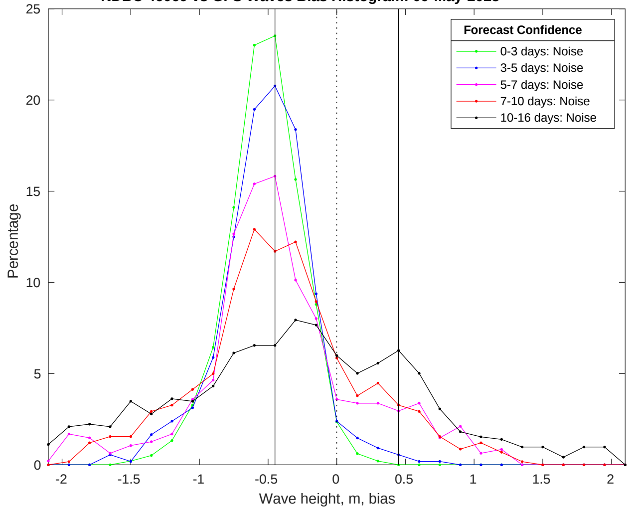
NDBC 46069 vs GFS Waves Bias Histogram: 09-May-2025
