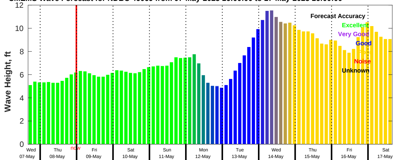
CMEMS Wave Forecast for NDBC 46069 from 07-May-2025 16:00:00 to 17-May-2025 16:00:00
