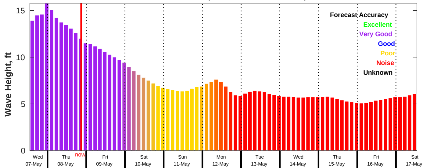
CMEMS Wave Forecast for NDBC 51209 from 07-May-2025 13:00:00 to 17-May-2025 13:00:00
