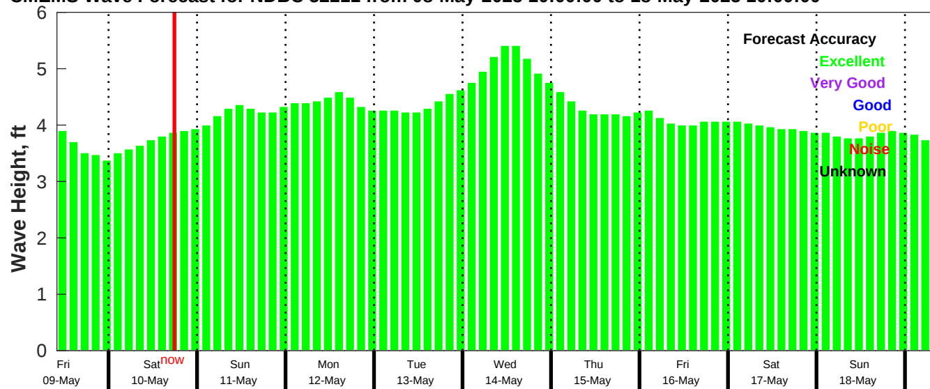
CMEMS Wave Forecast for NDBC 52211 from 08-May-2025 10:00:00 to 18-May-2025 10:00:00
