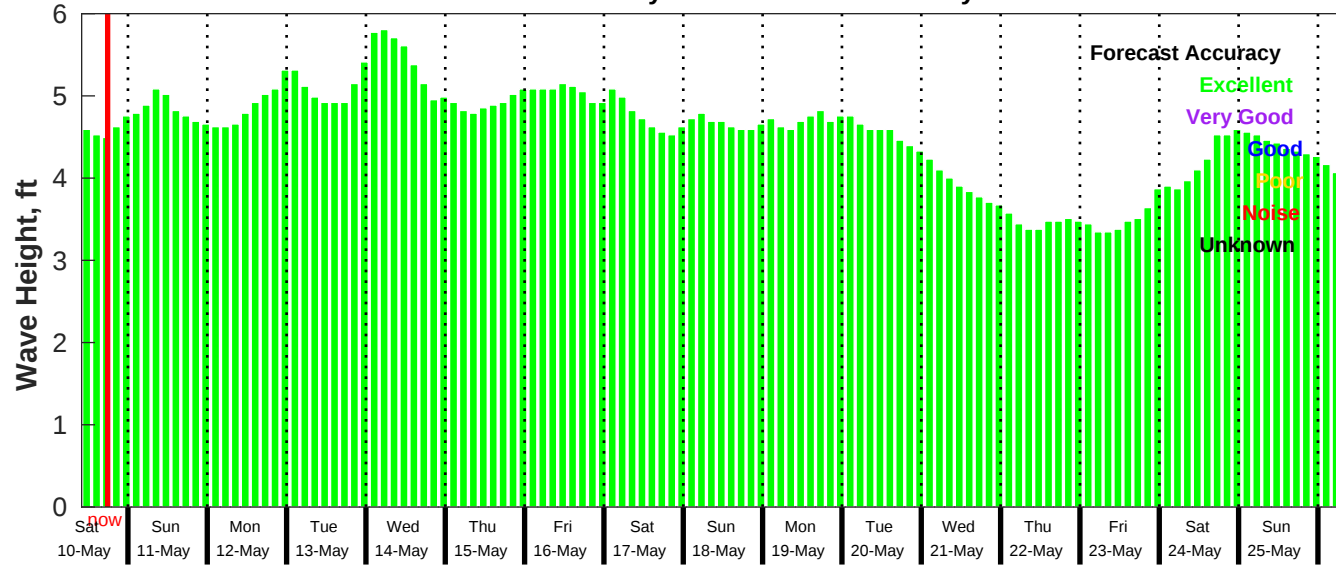
GFS Wave Forecast for NDBC 52211 from 09-May-2025 10:00:00 to 25-May-2025 10:00:00
