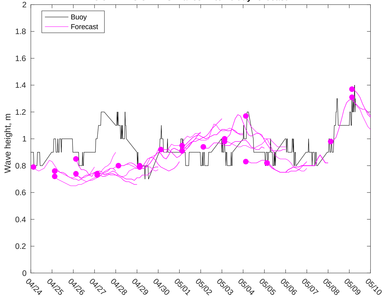
NDBC 52212 vs CMEMS Waves: 7 to 10 day forecast
