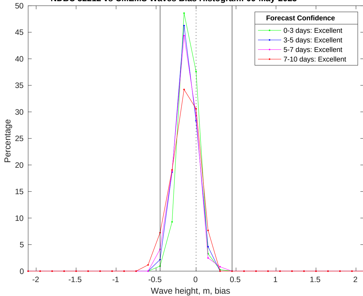
NDBC 52212 vs CMEMS Waves Bias Histogram: 09-May-2025
