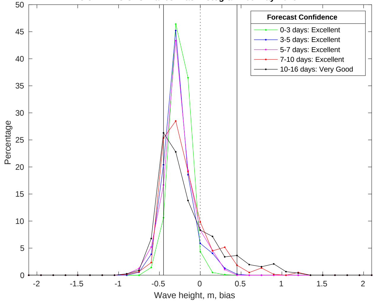
NDBC 52212 vs GFS Waves Bias Histogram: 09-May-2025
