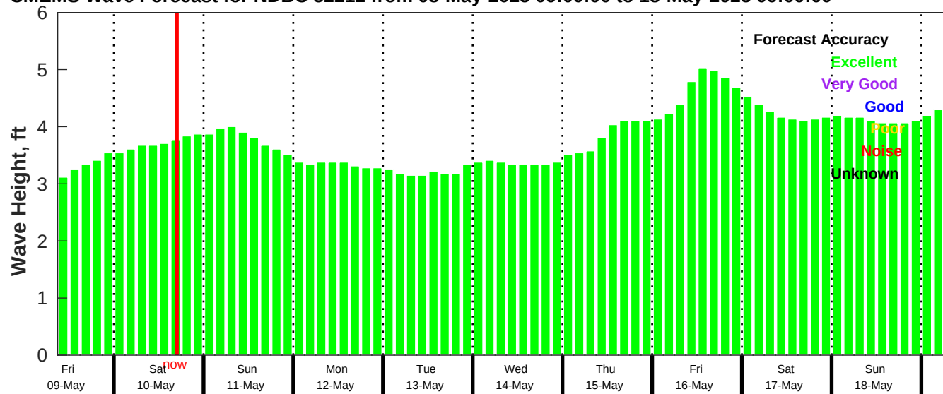
CMEMS Wave Forecast for NDBC 52212 from 08-May-2025 09:00:00 to 18-May-2025 09:00:00
