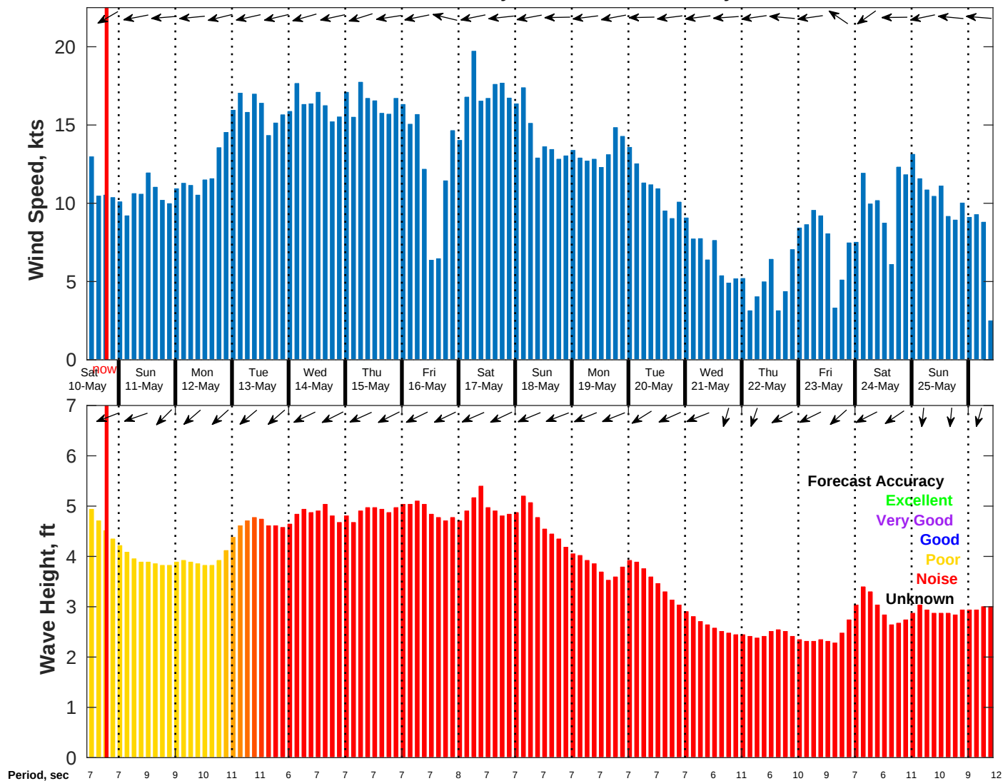
Wind & Wave Forecast for NDBC 52213 from 09-May-2025 11:00:00 to 25-May-2025 11:00:00
