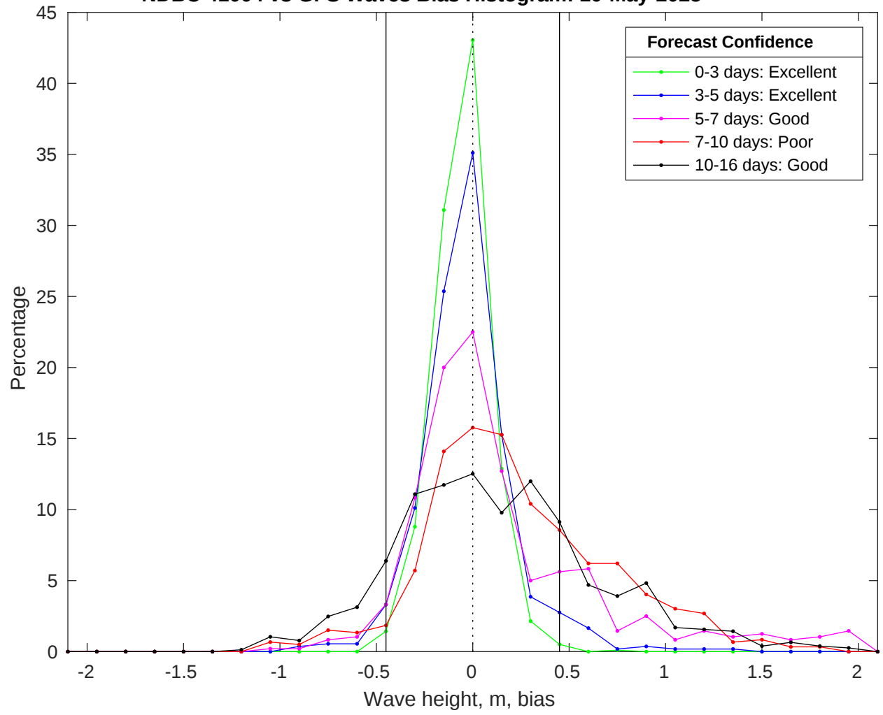
NDBC 41004 vs GFS Waves Bias Histogram: 10-May-2025
