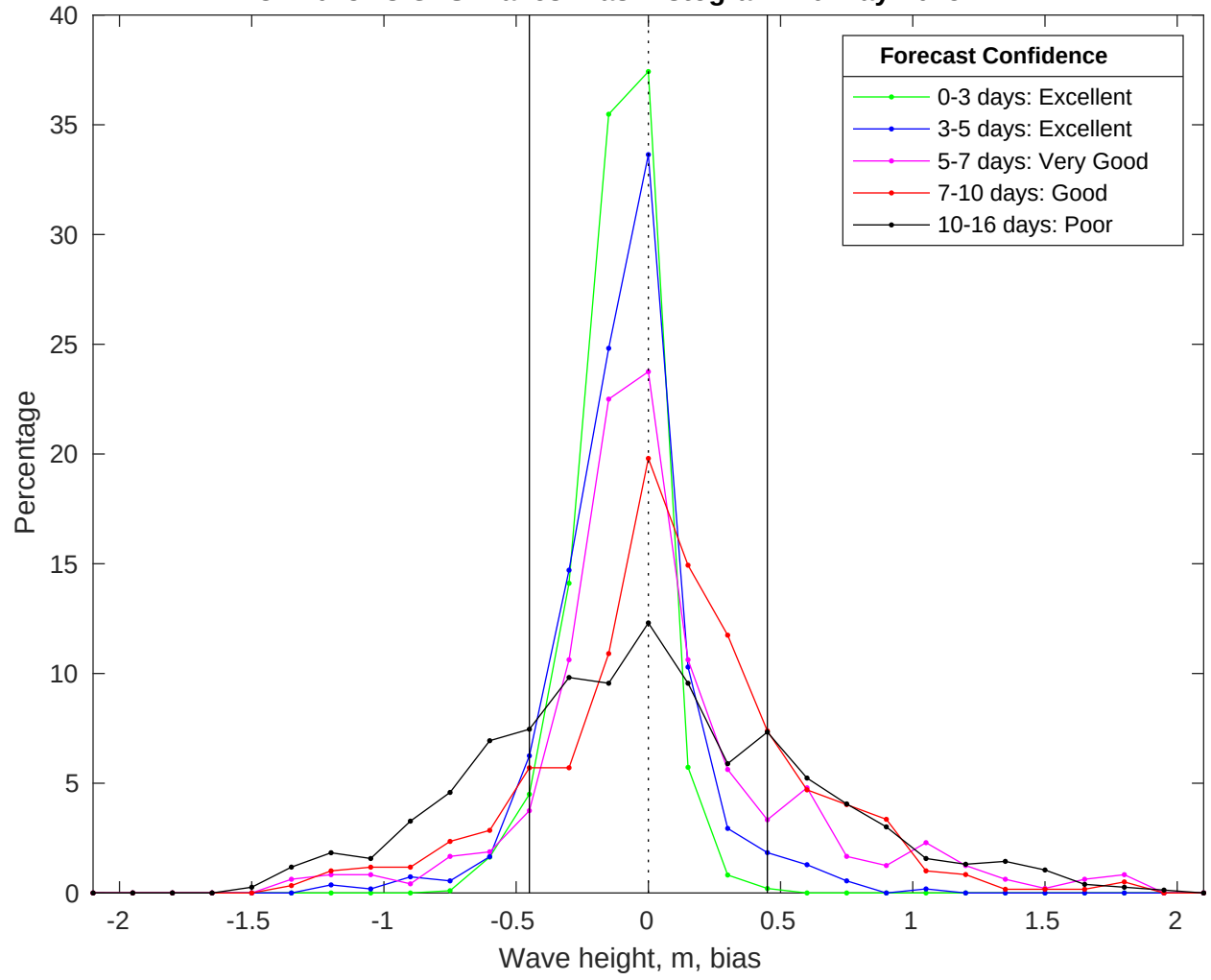
NDBC 41013 vs GFS Waves Bias Histogram: 10-May-2025
